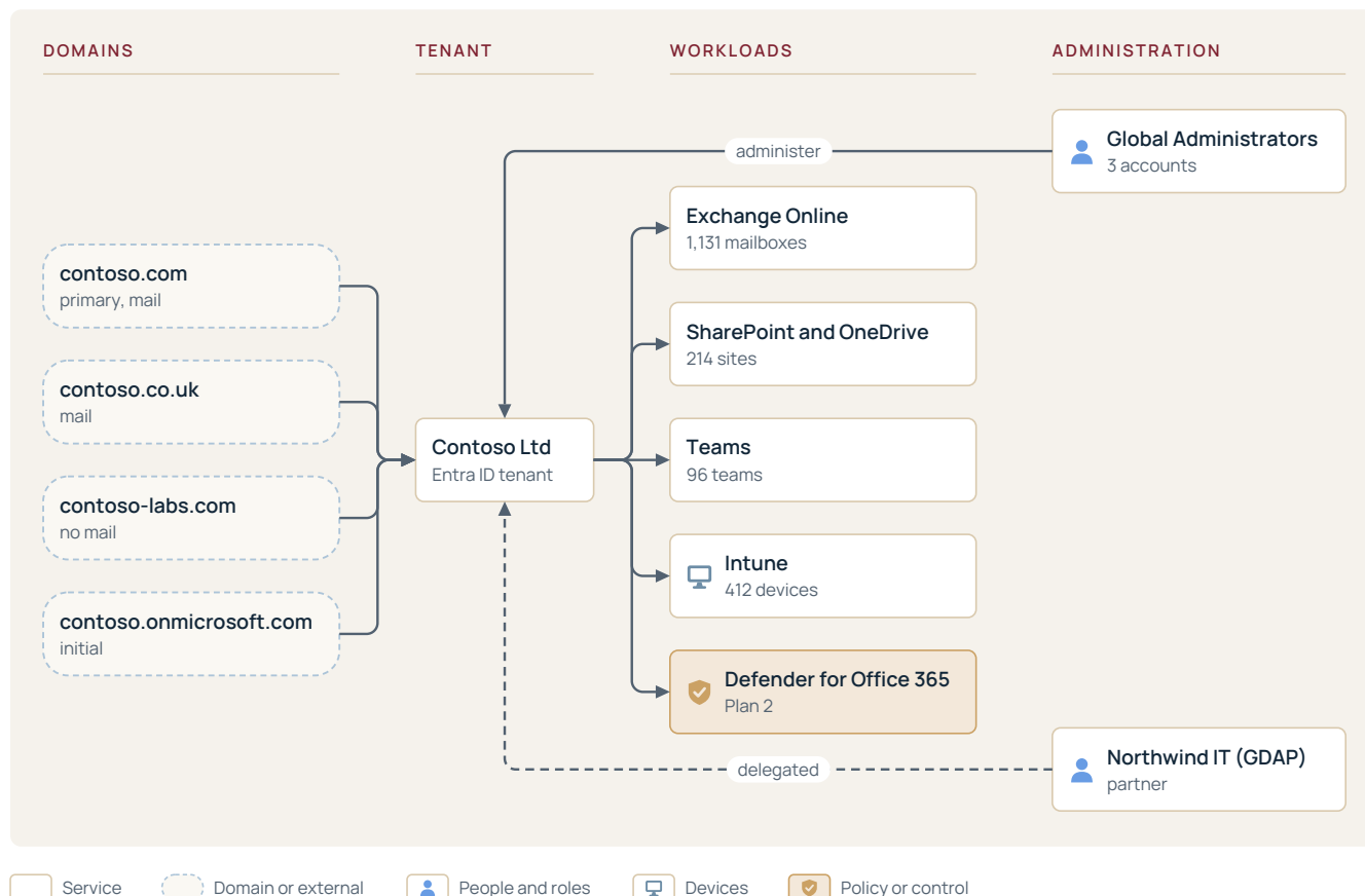
Figure 1. Tenant topology: domains, workloads in use and administration
