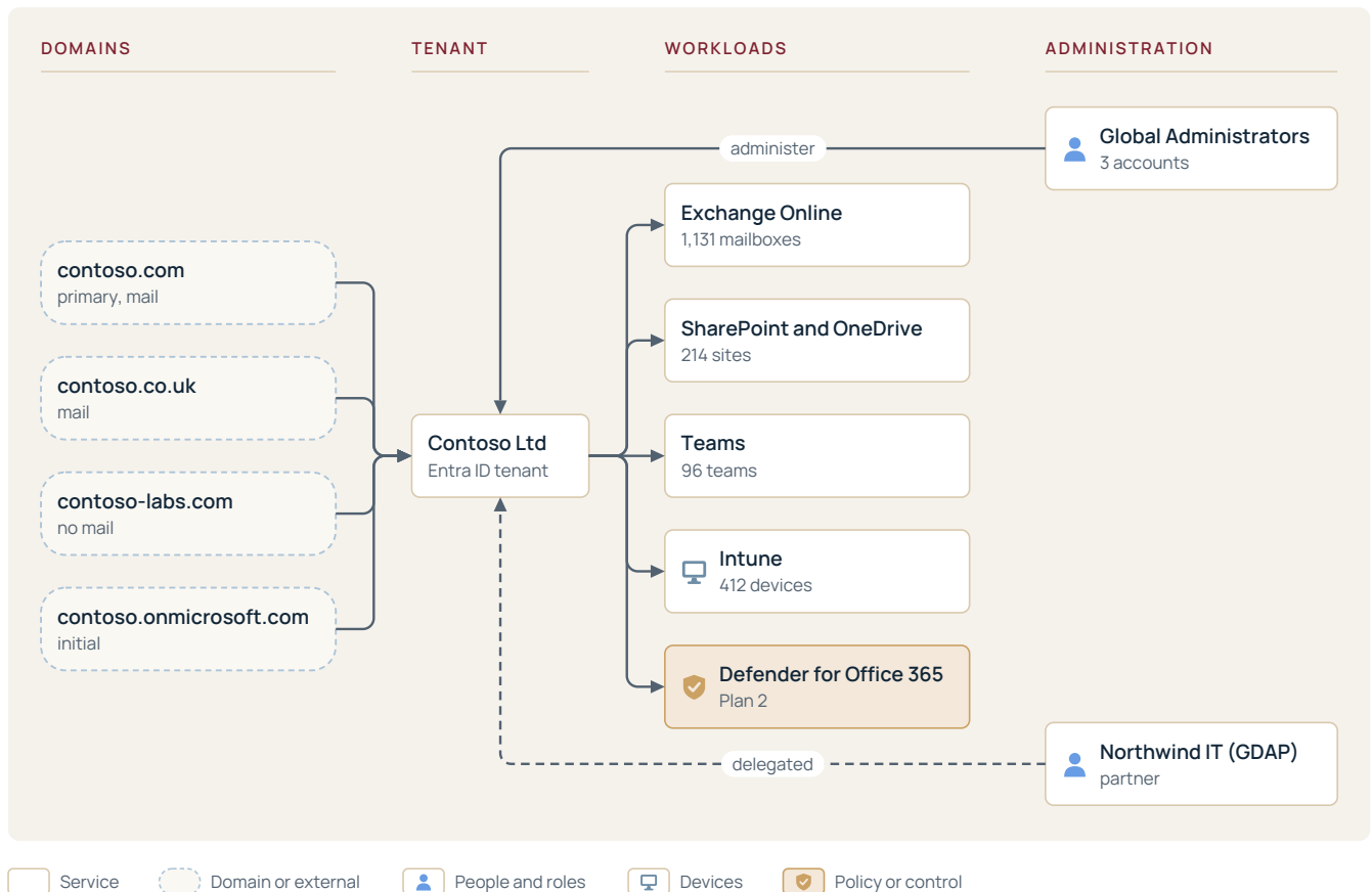
Figure 1. Tenant topology: domains, workloads in use and administration
