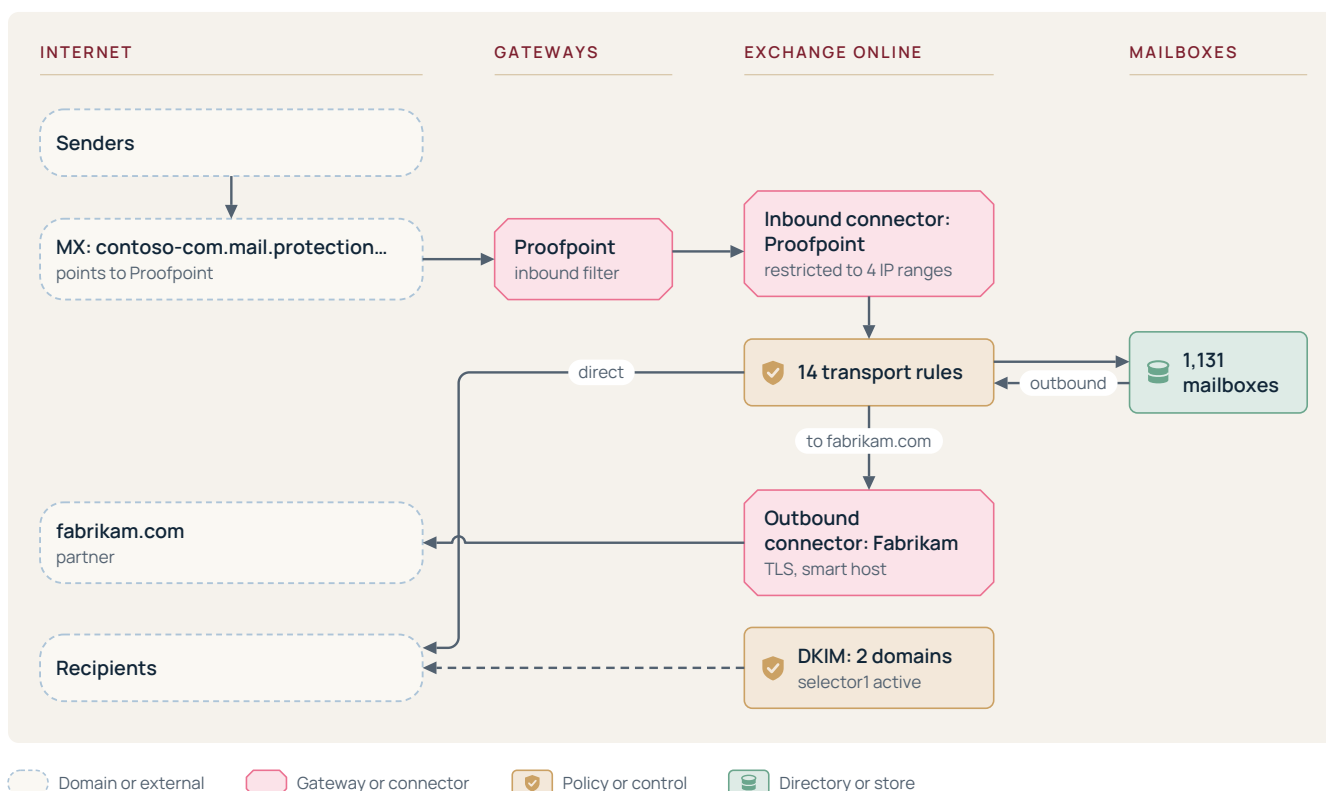
Figure 4. Mail flow: inbound and outbound paths
